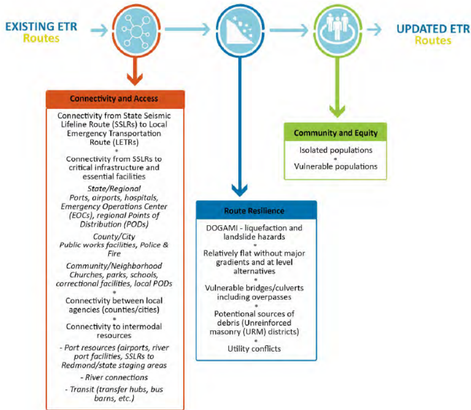
Figure 2: Evaluation Framework
