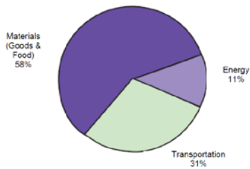
Figure 3.7: Major Sources of Eugene-Springfield Greenhouse Gas Emissions 20
